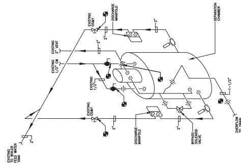
ISOMETRIC PIPING SCHEMATIC OF VACUUM CONDENSING UNIT
